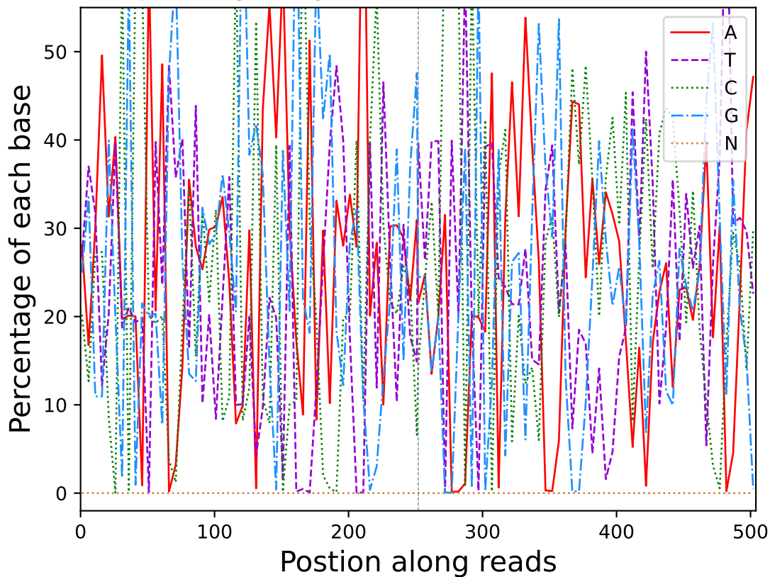
Base percentage along reads (R10423)
